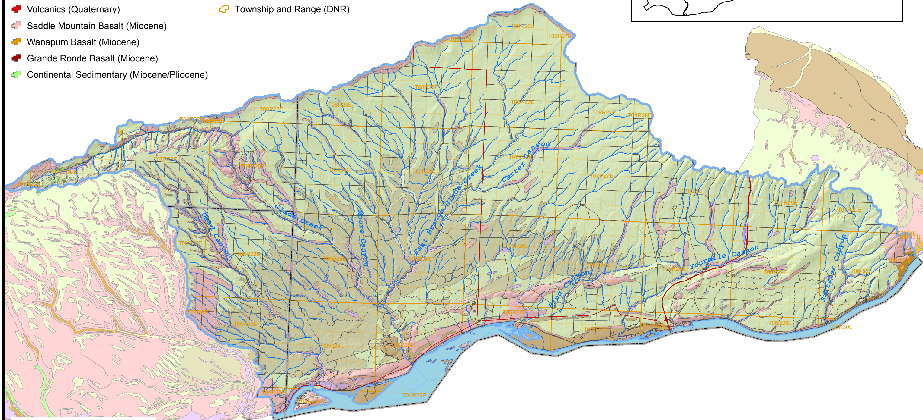
Figure 1 GEOLOGIC MAP GLADE/FOURMILE SUBBASIN WRIA 31 Level 2 Water Quality Project
