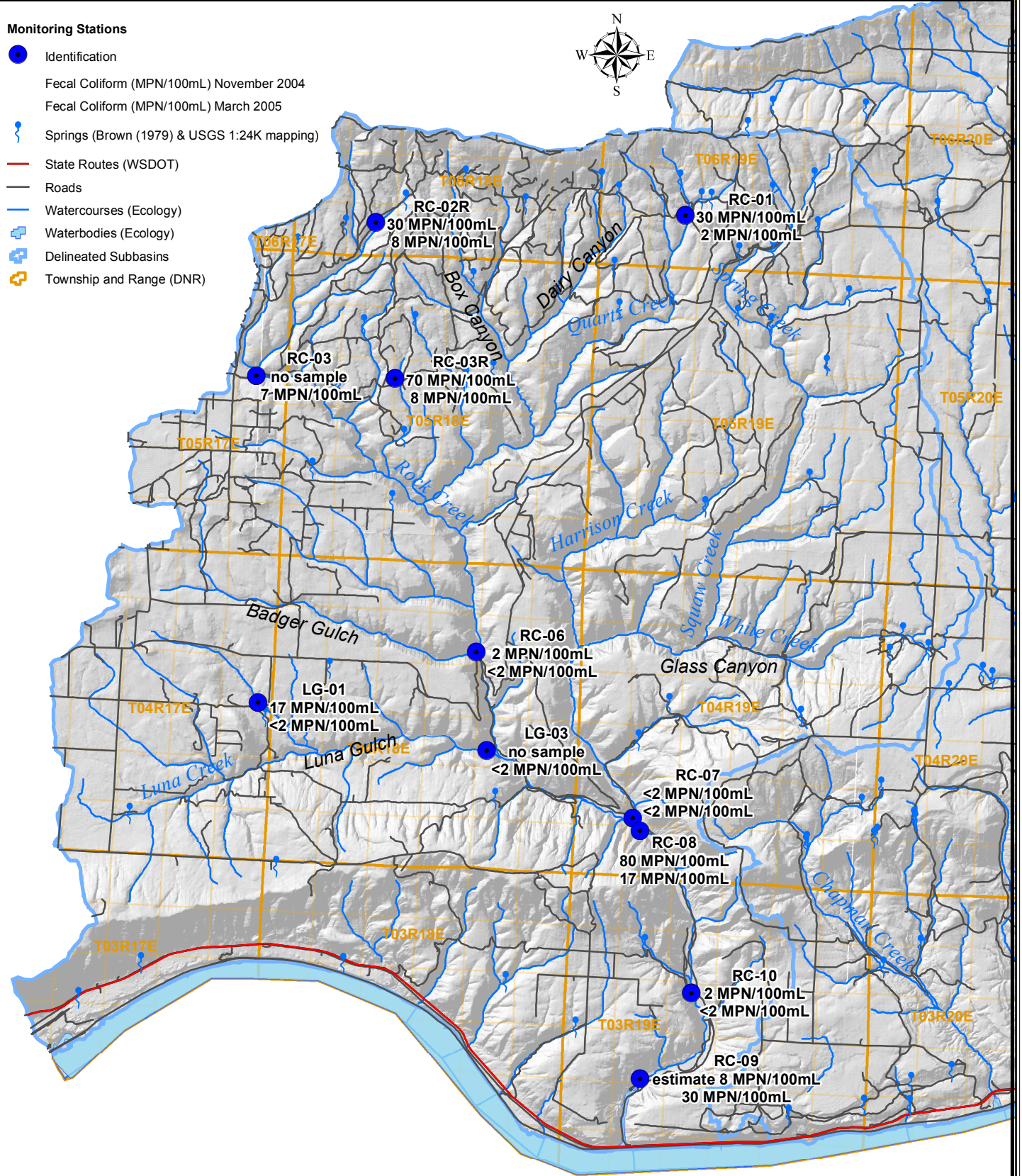
Figure 6 DISTRIBUTION OF FECAL COLIFORM CONCENTRATIONS IN ROCK CREEK SUBBASIN WRIA31 Level 2 Water Quality Project
