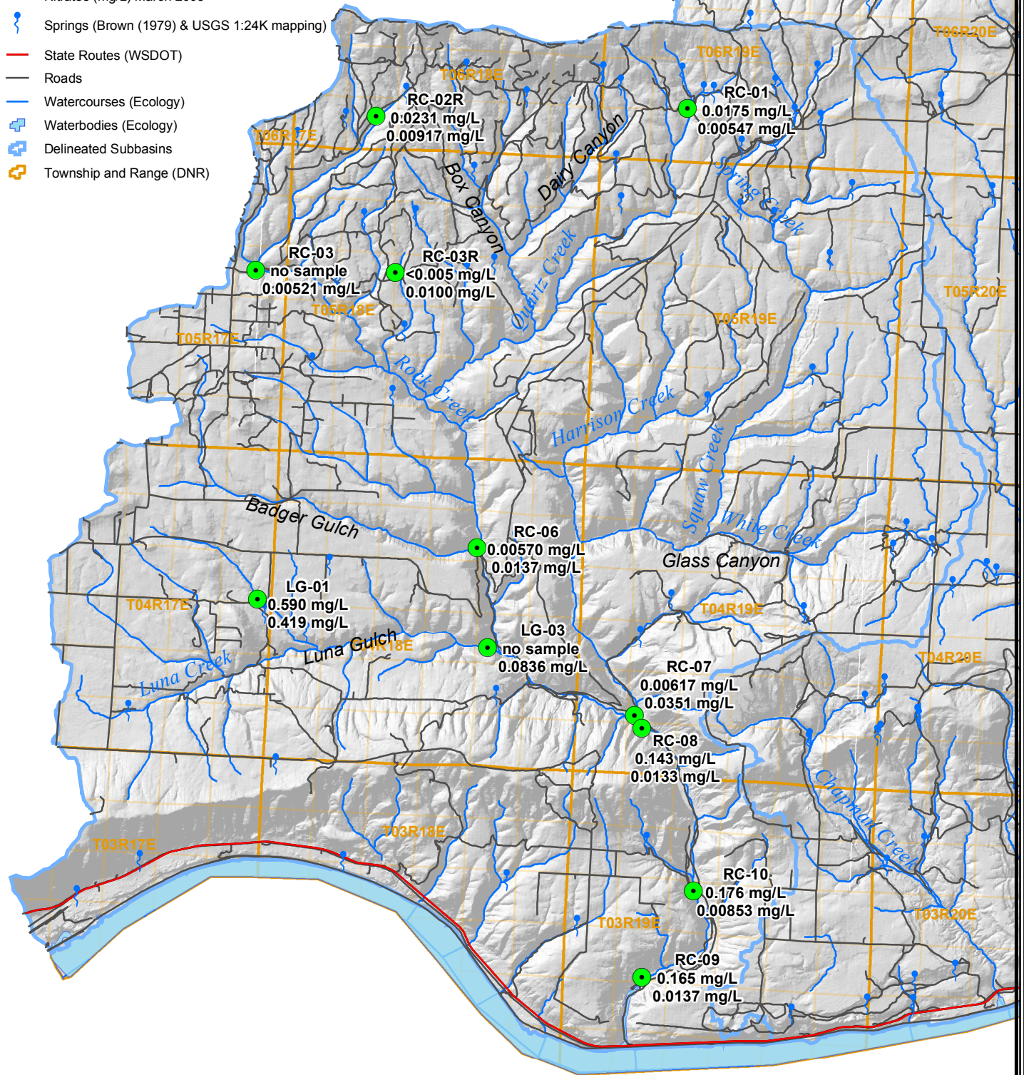
Figure 5 DISTRIBUTION OF NITRATE CONCENTRATIONS IN ROCK CREEK SUBBASIN WRIA31 Level 2 Water Quality Project
